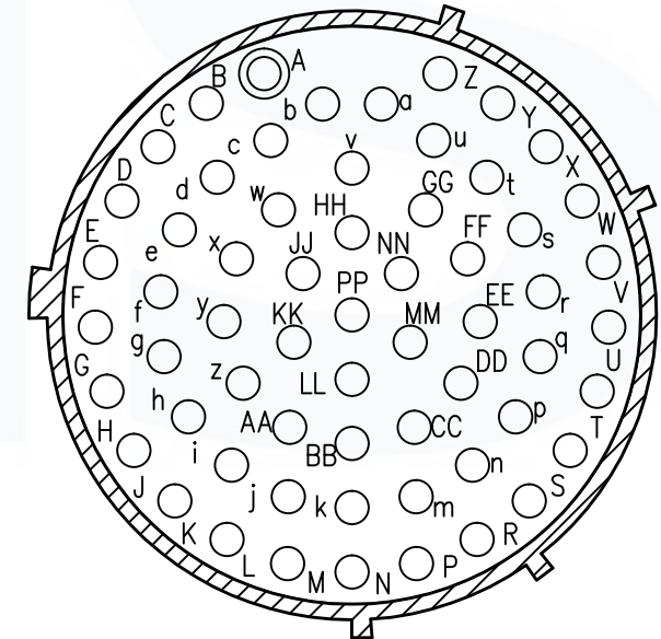
Pin Configuration
