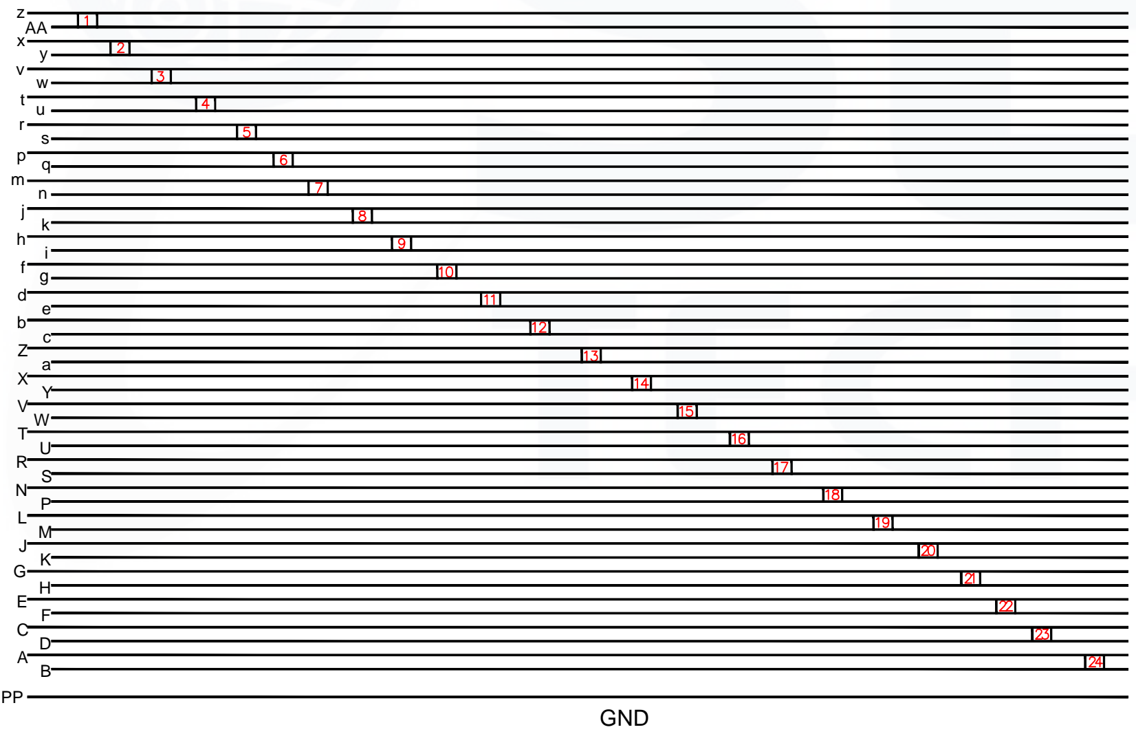
24Channel Hydrophone Cable Wiring Diagram
