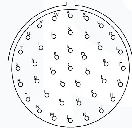
20-41P Connector Face View
